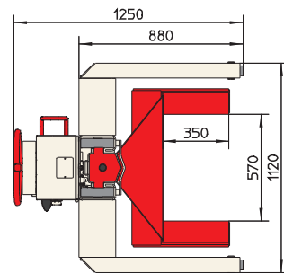
Fixed fork
