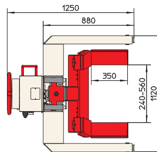
Adjustable fork
